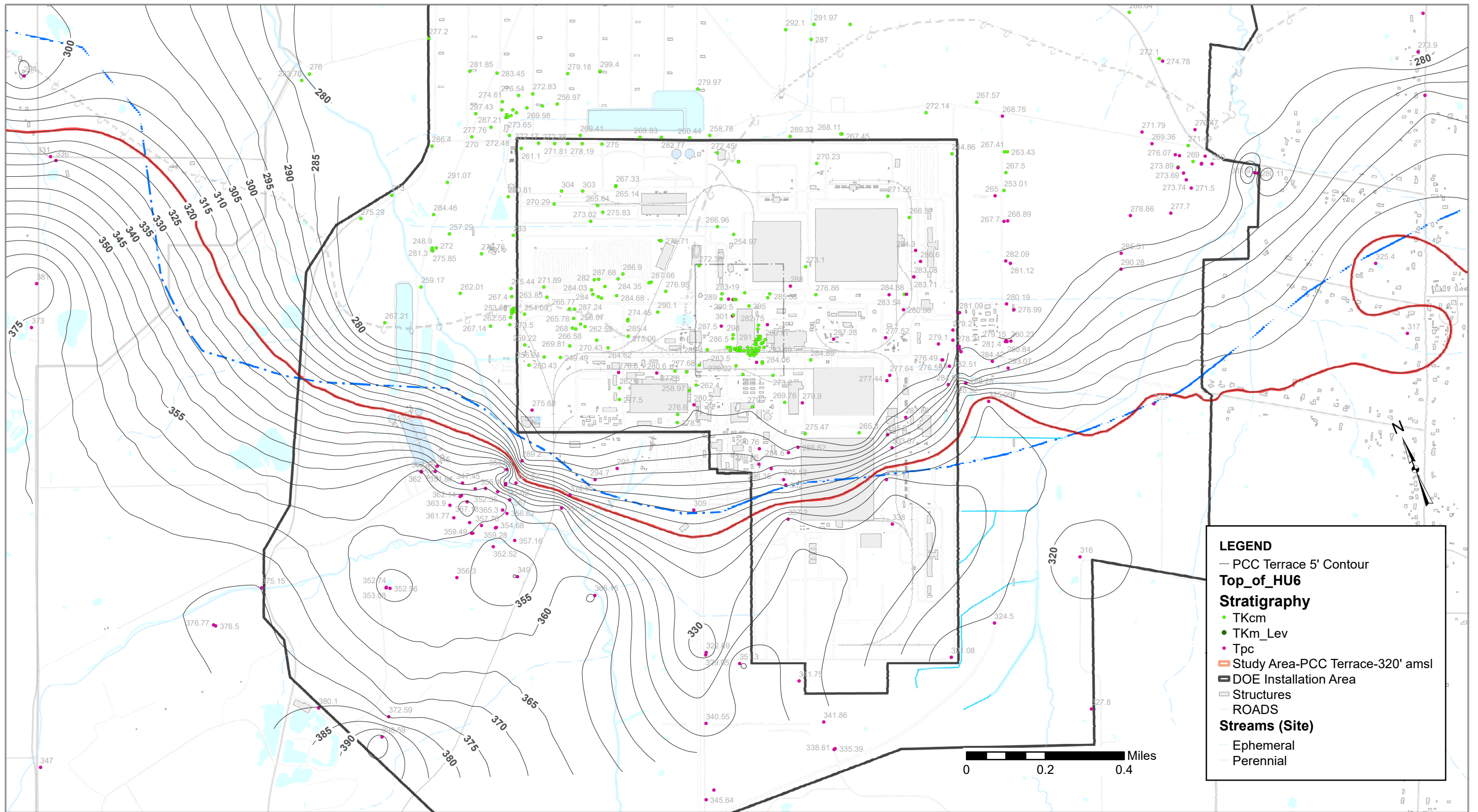
Figure 3. R10 Porters Creek Clay Terrace - DOE Property Interpolation: Ordinary Kriging Grid Spacing: 5'; Surface Contour Interval 5'; Smoothing: Focal Statistics (ESRI)
