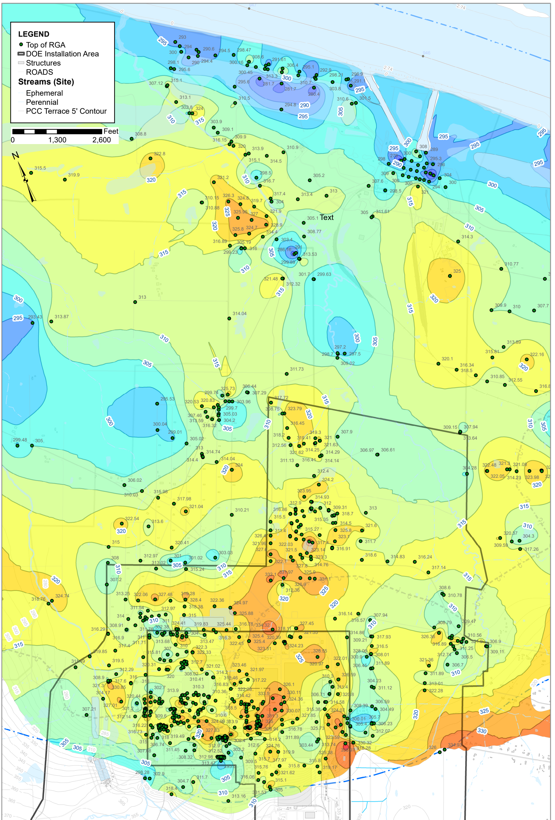
Figure 4. R10 Top of RGA - DOE Site to TVA Interpolation: Ordinary Kriging; Grid Spacing: 5'; Surface Contour Interval 5' Smoothing: Focal Statistics (ESRI)
