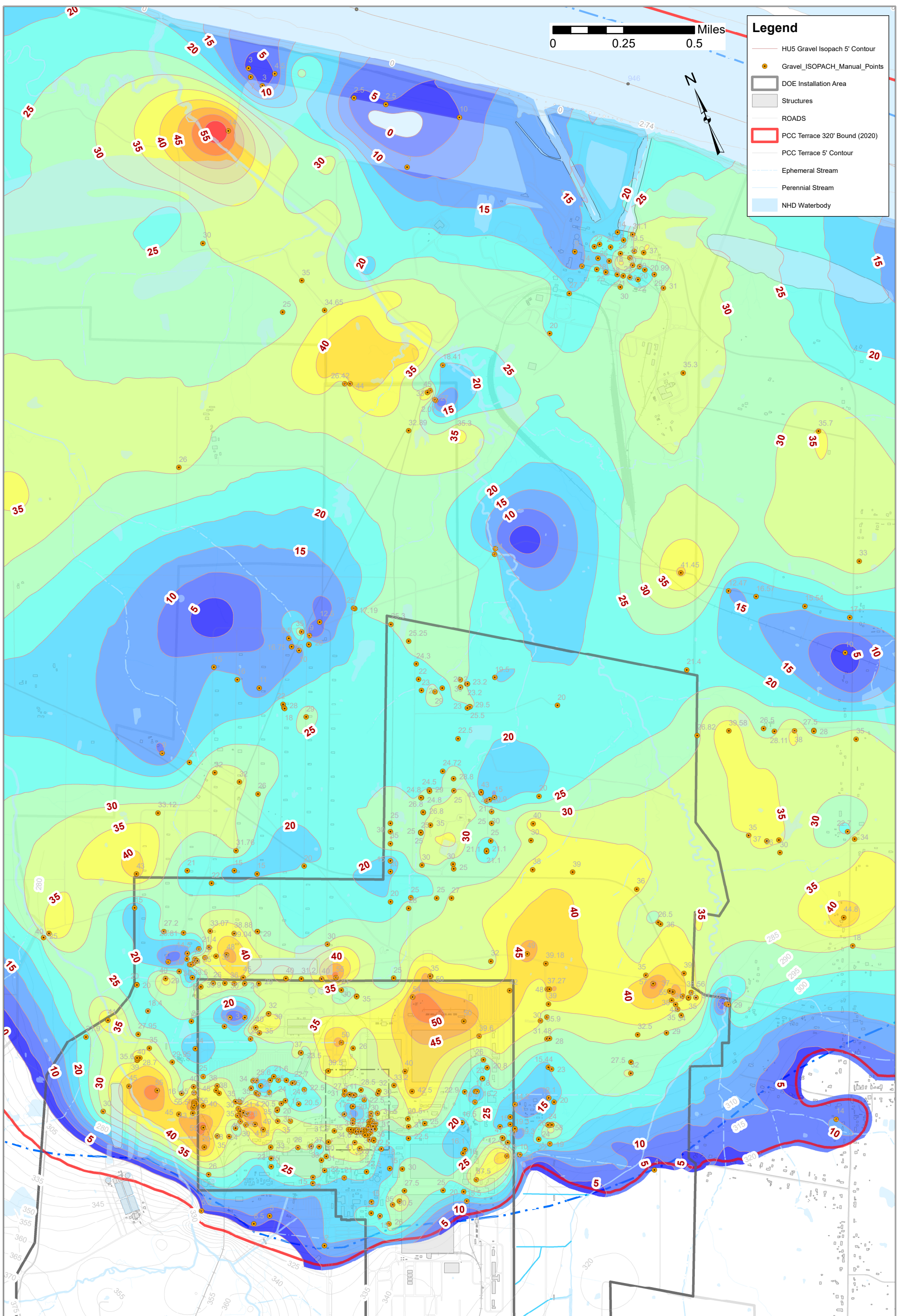
Figure 5a. R10 RGA Gravel Isopach - DOE-TVA Interpolation: Ordinary Kriging; Grid Spacing: 5'; Surface Contour Interval 5'; Smoothing: Focal Statistics (ESRI)
