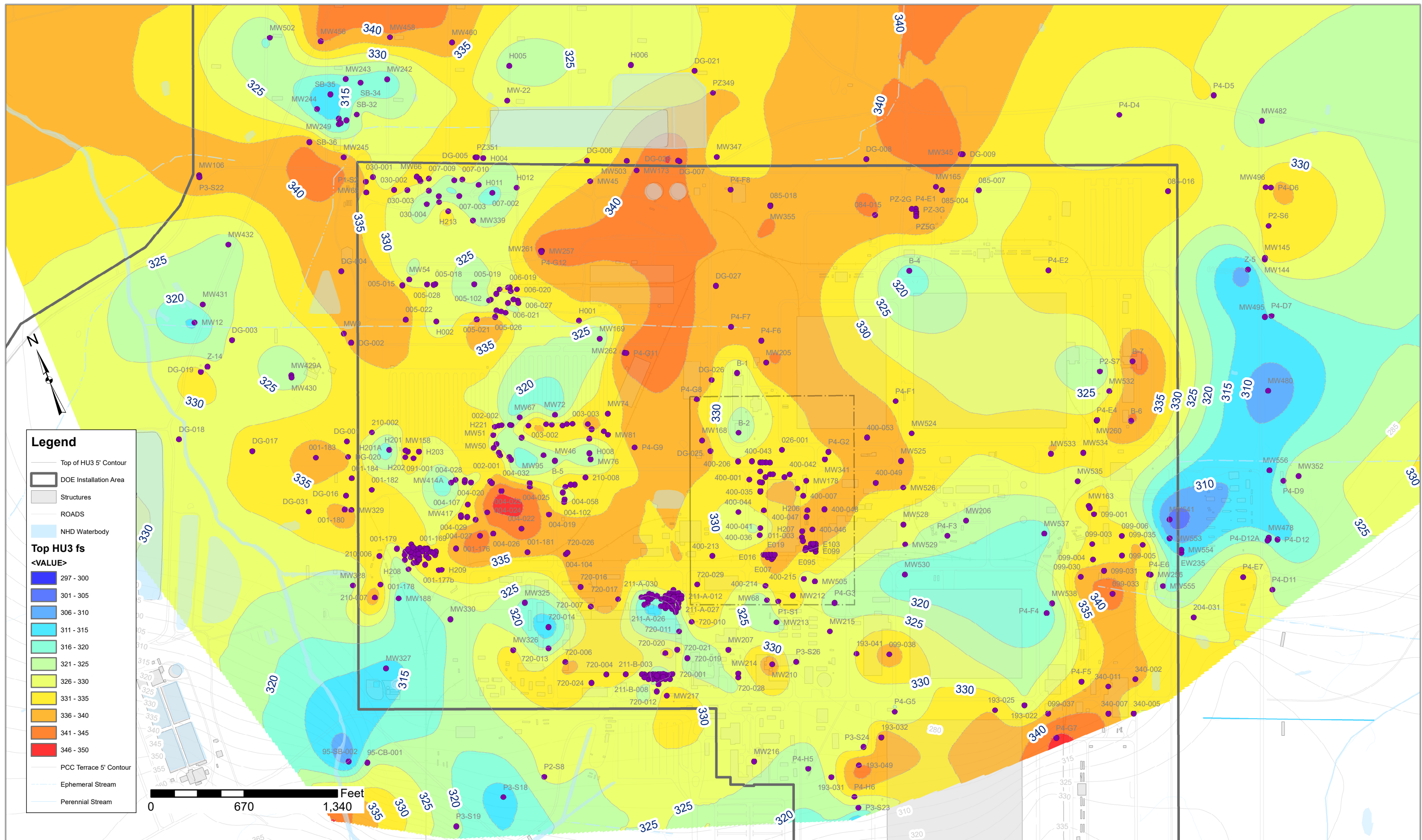
Figure 6. R10 Top of HU3 - Industrial Site Interpolation: Ordinary Kriging; Grid Spacing: 5'; Surface Contour Interval 5'; Smoothing: Focal Statistics (ESRI)
