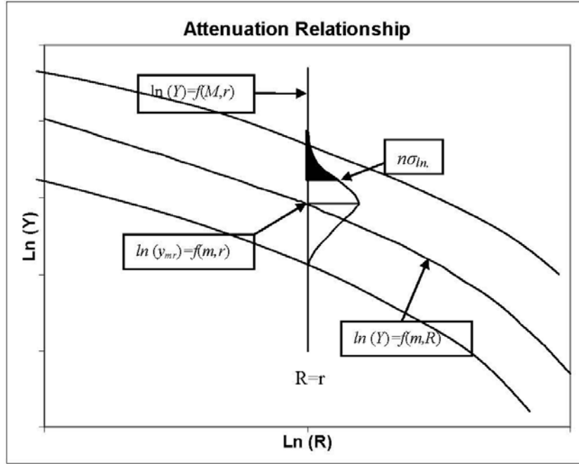
Figure 2. Ground-motion attenuation relationship.
