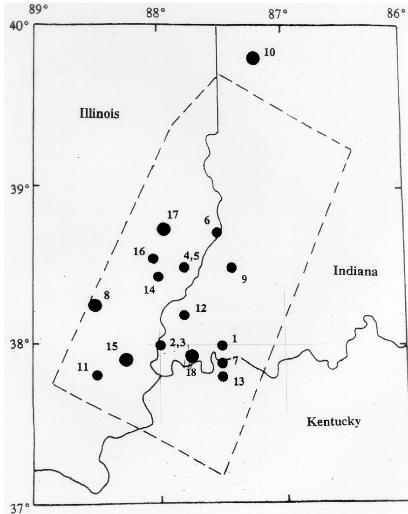
Figure 10. Epicentral locations of the felt earthquakes in the Wabash Valley Seismic Zone.
