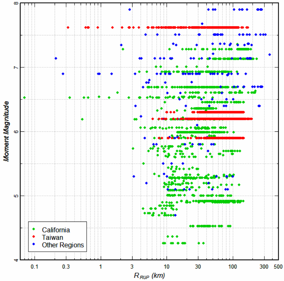
Figure 24. Magnitude-distance-region distribution of selected recordings (Chiou and Youngs 2006).
