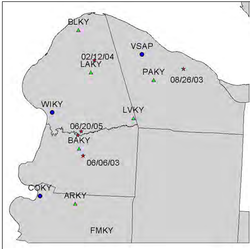
Figure 9. Seismic network and earthquakes (stars) recorded between January 2003 and June 2005 in the Jackson Purchase Region (Anderson and others 2005). Triangle – short-period seismic station; Circle – strong motion station.
