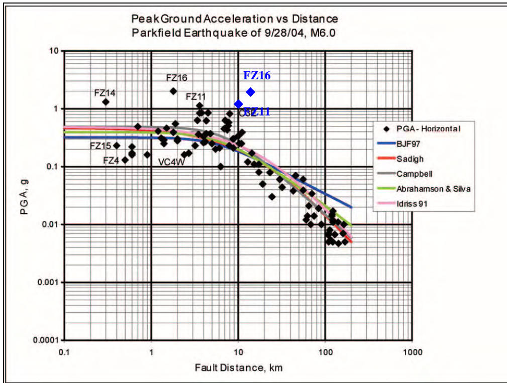
Figure 22. Horizontal uncorrected PGA vs. distance to the fault for the Parkfield earthquake of September 28, 2004 (Shakal and others 2006). Blue diamonds are plots for stations FZ11 and FZ16 if the epicentral distance is measured.
