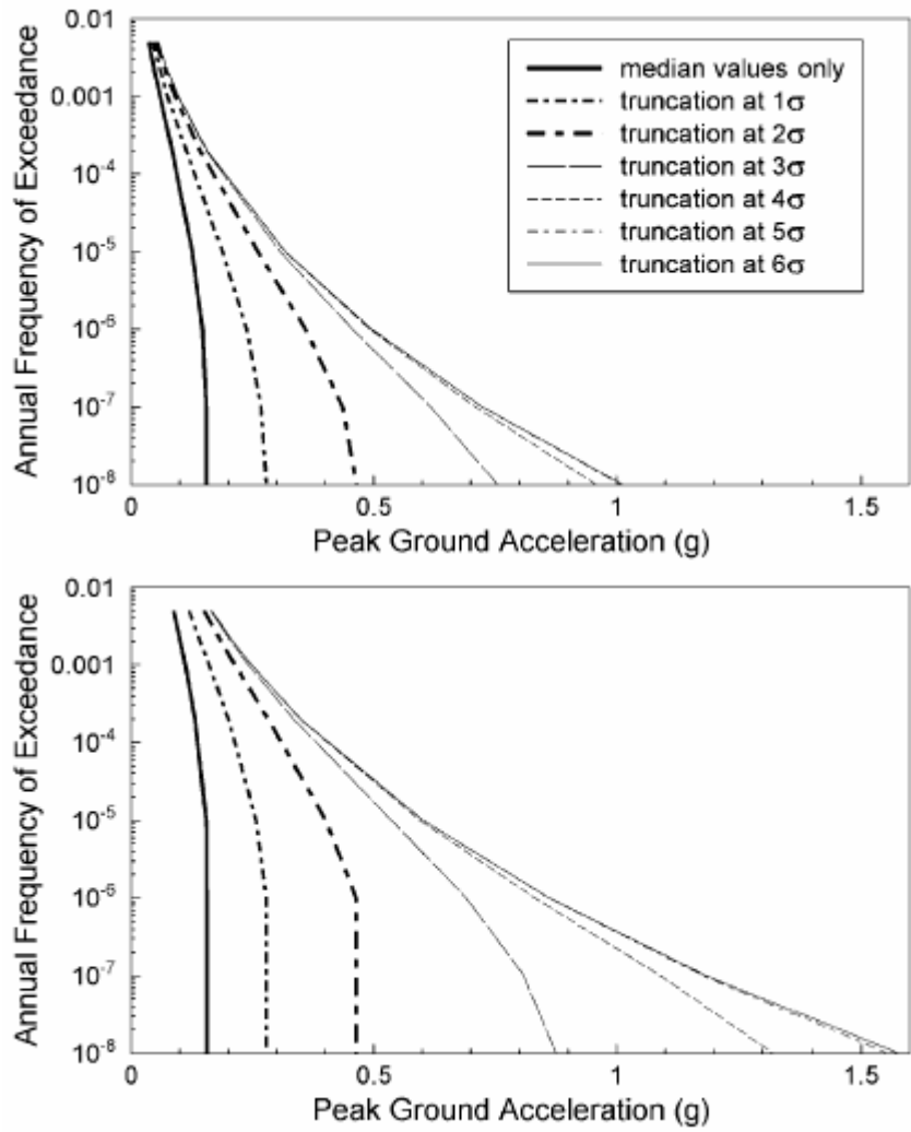
Figure 4. PGA hazard curves showing the effect of ground-motion uncertainty (Bommer and Abrahamson 2006).
