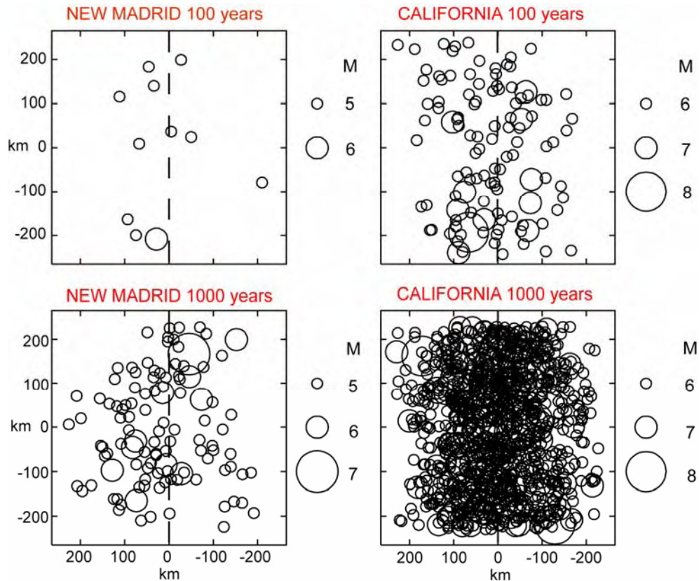
Figure 1. Schematic comparison of seismic hazard for the New Madrid Seismic Zone and southern California on two time scales. Circles mark area of shaking with acceleration > 0.2g (Stein and others 2003).
